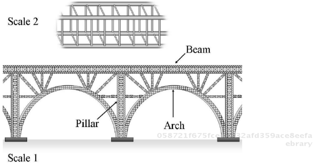
Figure 3. Bridge design applying the principle of structural hierarchy for bridge reinforcement.
