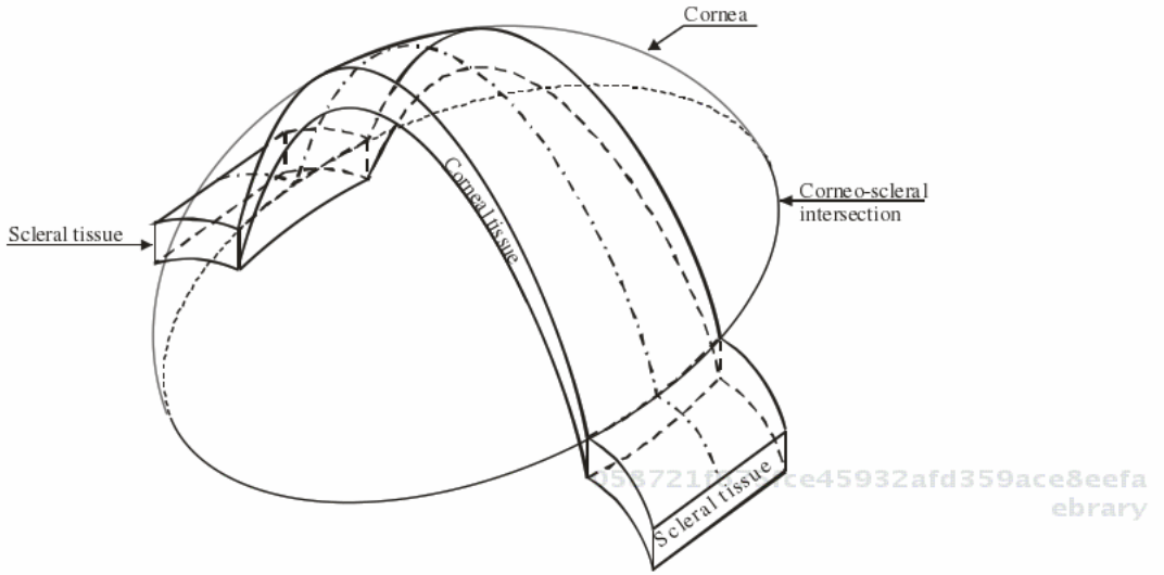
Figure 11. Initial curved form of corneal strip specimens.
