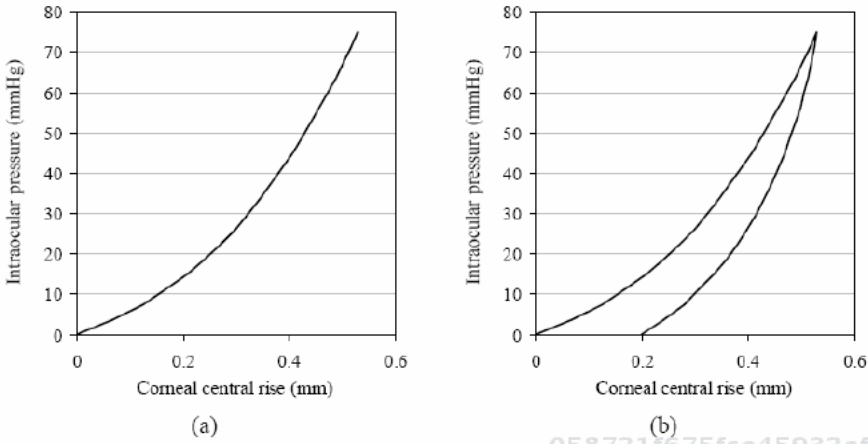
Figure 42. Model predictions of the behaviour of a cornea subjected to a cycle of pressure increase and decrease while (a) ignoring and (b) considering the unloading behaviour of corneal tissue.
