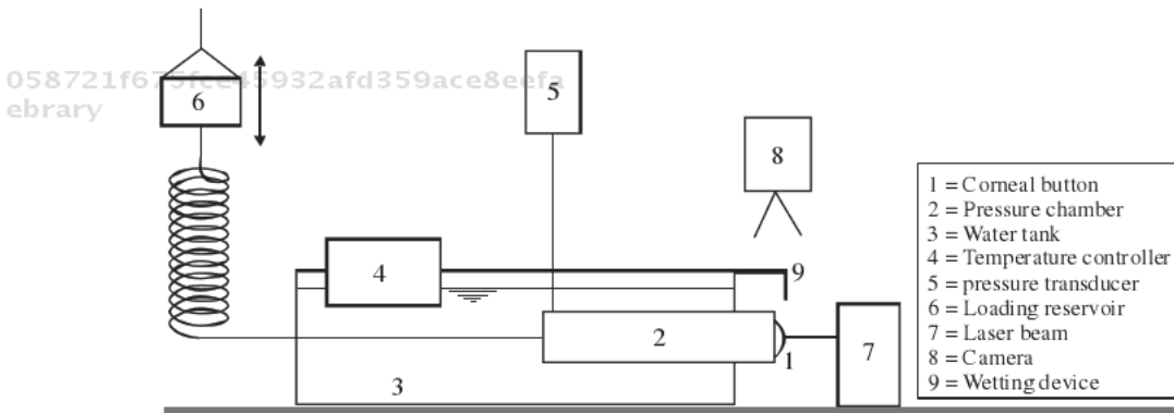
Figure 8. Main components of an inflation test rig.
