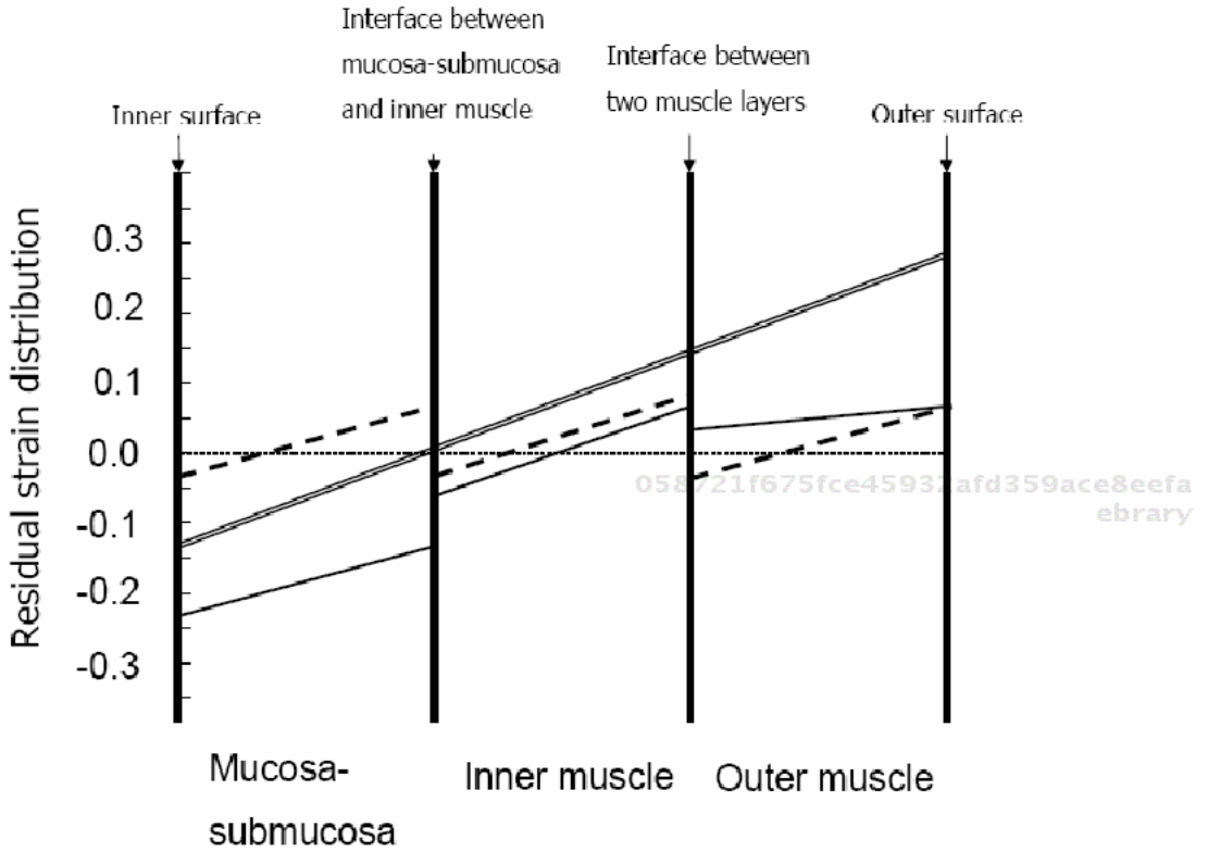
Figure 2. Residual strain distribution in the intact wall and layers of pig oesophagus. Residual strain distribution of the intact wall referenced to the zero-stress state of the intact wall Residual strain distribution of layered wall in intact wall referenced to the zero-stress state of layered sectors Residual strain distribution of separated layers referenced to the zero-stress state of layered sectors. Referenced to the zero-stress state of the intact sectors, the inner residual strain of intact rings was -0.13 \pm 0.04 and outer residual strain was 0.31 \pm 0.03 . Referenced to the “true” zero-stress state of separated three layered sectors, the inner residual strain of intact rings was -0.22 \pm 0.02 and outer residual strain was 0.07 \pm 0.02 . The residual strain distribution of the layers in intact rings referenced to the “true” zero-stress state is also shown. The inner surface residual strain was negative at mucosa-submucosa and inner muscle layers and was positive at outer muscle layer, whereas the outer surface residual strain was negative at the mucosa-submucosa layer and positive at the inner and outer muscle layers. Referenced to the “true” zero-stress state, the inner residual strain was negative and outer residual strain was positive for the separated layered rings.
