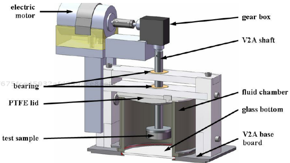
Figure 3. Adhesion measuring device adapted to be used in conjunction with a LSM shown schematically.
