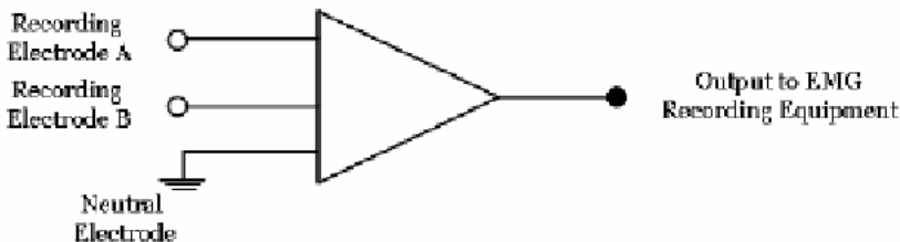
Figure 3. Schematic representation of a monopolar vs. bipolar electrode configuration. Monopolar recordings consist of a single electrode being placed on or in the muscle of interest while a second neutral (reference/ground) electrode being placed at an electrically quiescent site (e.g., bone), whereas bipolar recordings consist of two electrodes being placed on or in the muscle of interest along with a neutral electrode.
