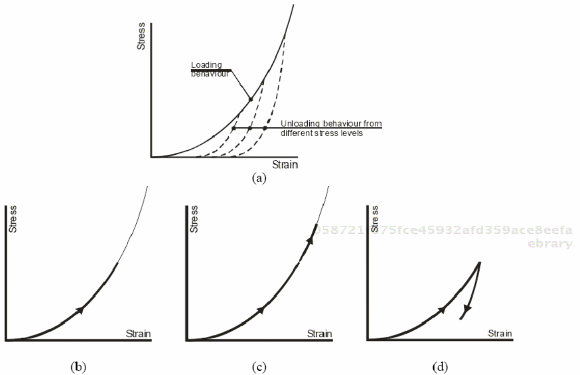
Figure 41. (a) Behaviour of corneal tissue under both loading and unloading conditions, and the stress development in a particular element during an FE analysis including (b) the stress history, and the behaviour adopted if the element is to undergo either (c) further loading or (d) unloading.
