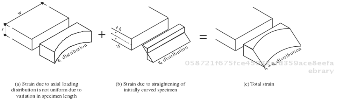
Figure 14. Strain distribution on the cross-section of a strip specimen.
